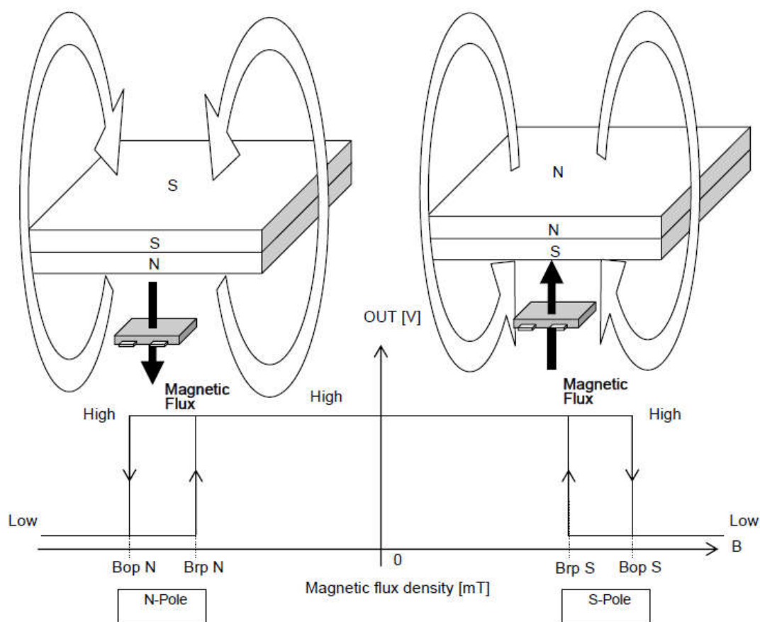
Fig 4, Magnetic Operation Characteristic of AS1820
