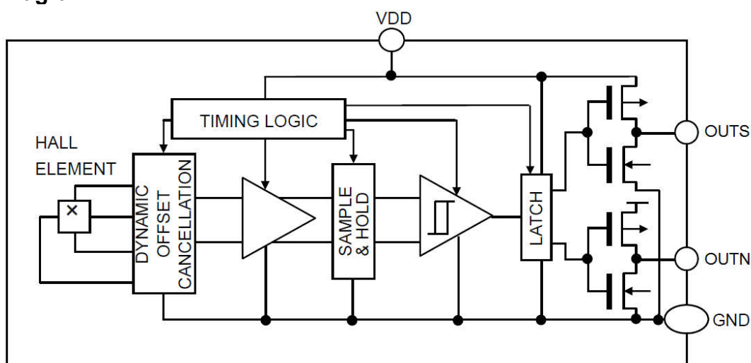
Figure 3, Block Diagram of AS1820
