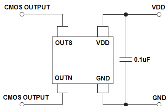
Figure 1, Typical Application Circuit of AS1820
